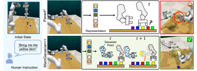
Fig. 1. Consider the human instruction “Bring me the yellow item”, where the task is considered successful if the right arm handover the yellow block to the left arm. The previous method (Peract 2 [15]) attempts to pick up the yellow block but fails to do so, while our ManiGaussian++ completes the task successfully by explicitly encoding the scene dynamics via future scene reconstruction in Gaussian embedding space.
