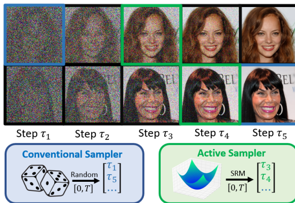
(b) Active Calibration TimeStep Selection
