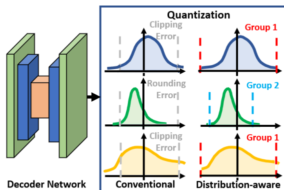
(a) Distribution-aware Quantization
